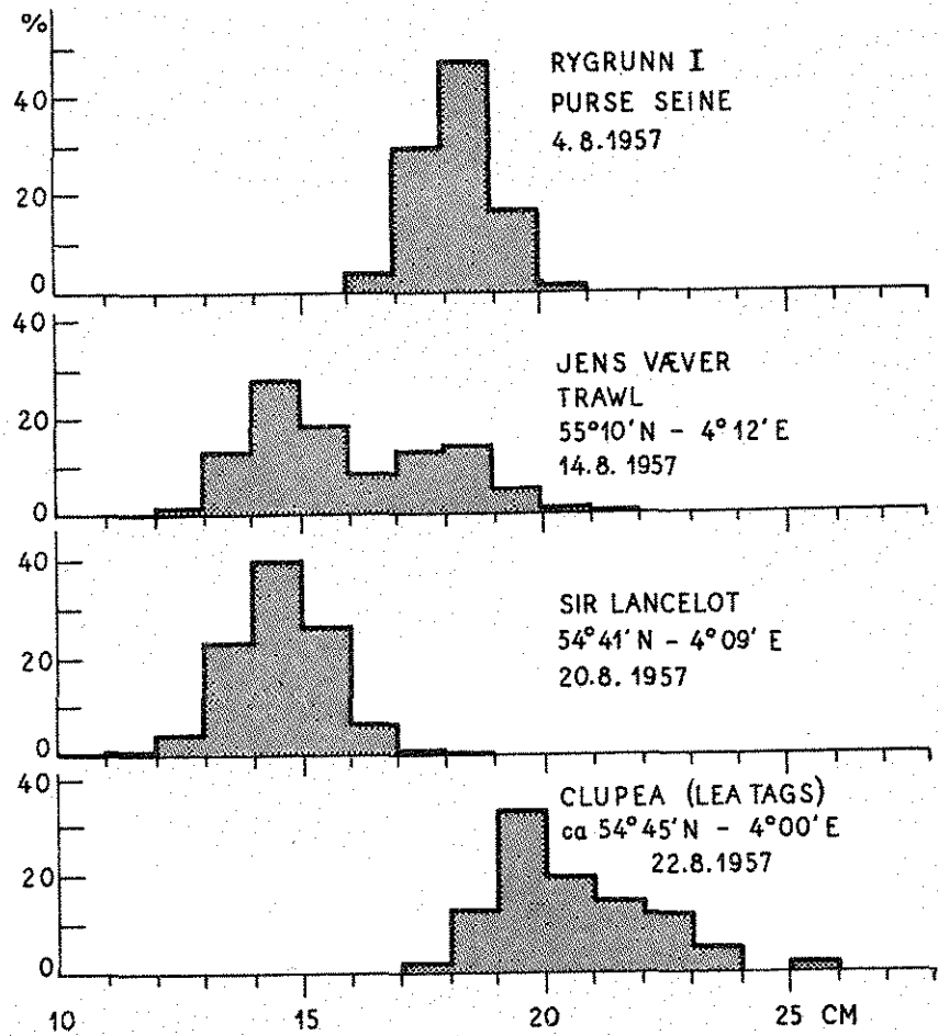
FIG. 5: Percentage length distribution of tagged herring.
