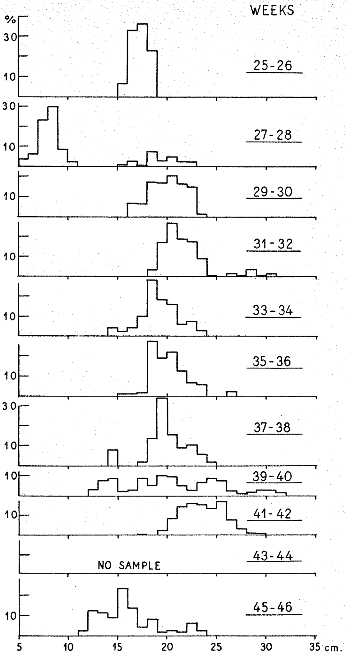
FIG. 4: Percentage length distribution of herring landed in each 2-week period at Esbjerg 1957. (Data from K. Popp Madsen MS)
